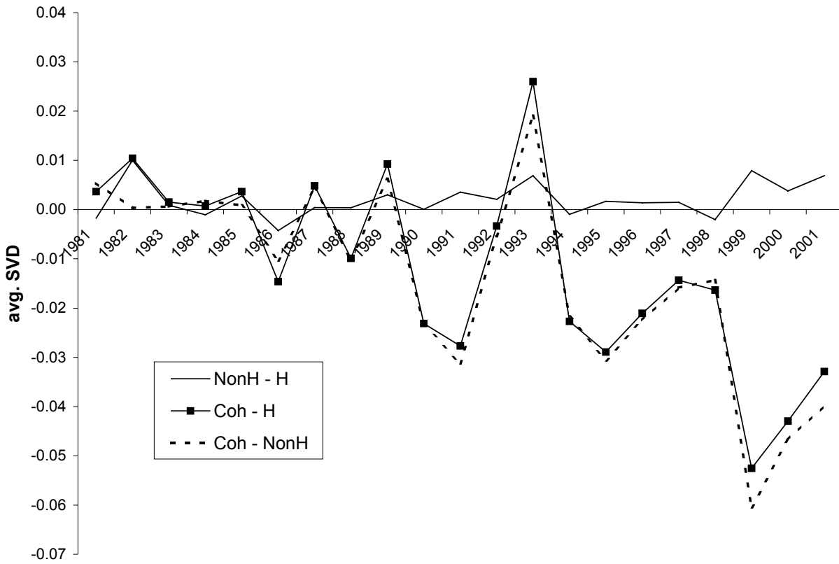
Figure 4: Avg. SVD Distance Metric: Annual Mobility Matrices, Cohort, Homogeneous and Non-Homogeneous Duration. Matrices estimated using S&P rated U.S. obligors, 1981-2001.
